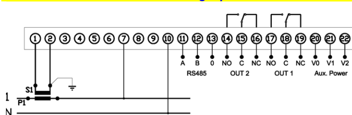
Circuito monofase / Single-phase circuit
