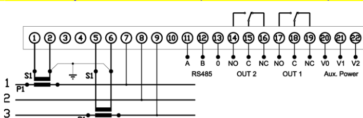
Circuito trifase a 3 fili (2 TA, inserzione ARON) Three-phase 3 wires circuit (2 CT, ARON insertion)
